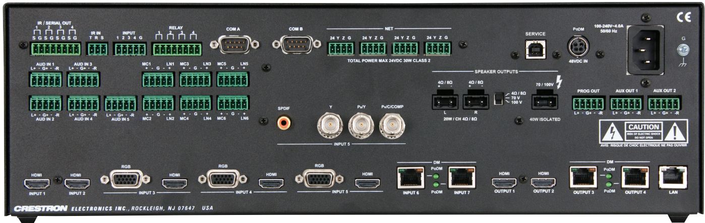
DMPS-300-C-AEC – Rear View
